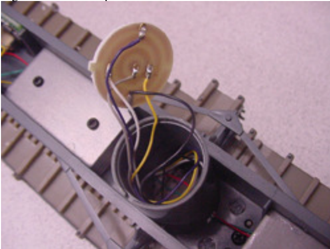
Figure 3: Removing PCB
