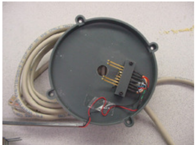
Figure 12 – Drill Hole
