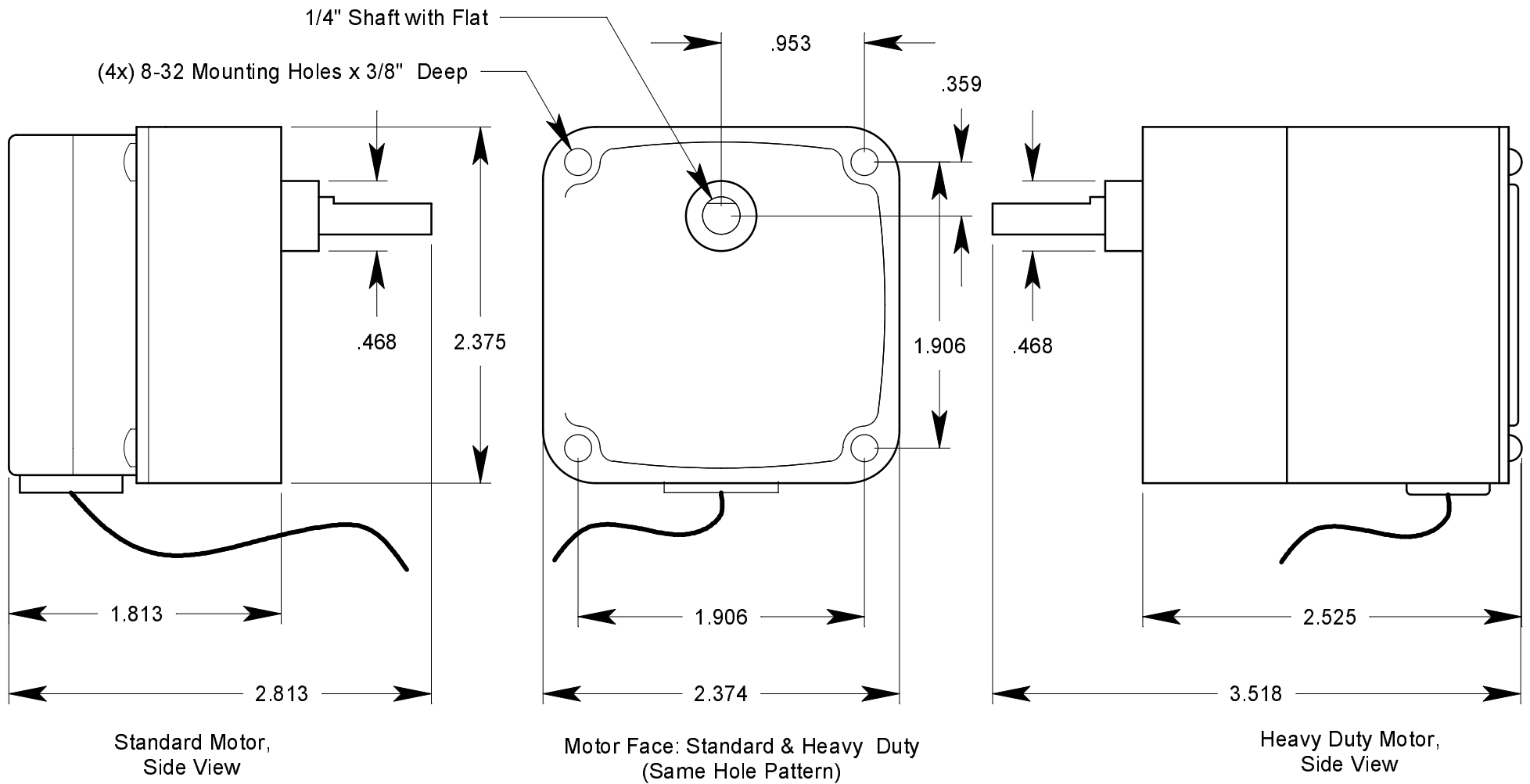
Figure 1: PTC Model III Motor Dimensions Standard and Heavy Duty Models. Not to Scale.
