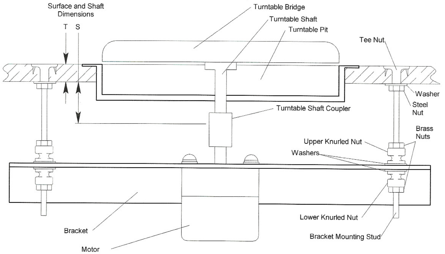
Figure 1: Motor Mount Cross Section (Not to Scale)
