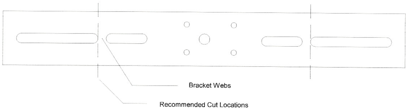
Figure 2: Mounting Bracket Top View (Not to Scale)
